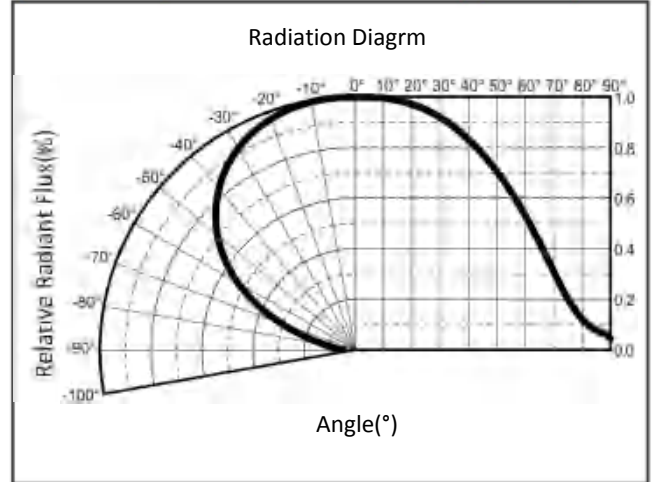
e) Beam Angle Characteristics 光束角 ( T_j = 25^\circ\text{C} )
